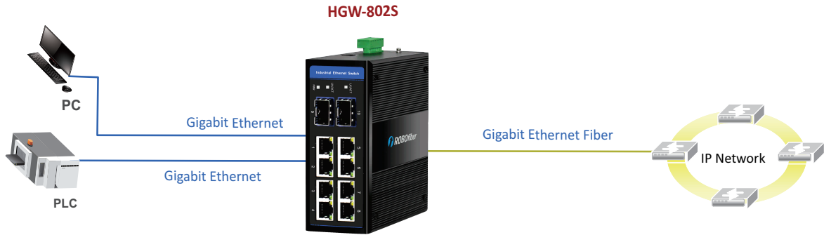
HGW-802S Gigabit Ethernet Switch Application
