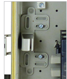
Single and Dual Hurricane Fiber Clips installed in WAVE enclosures.
